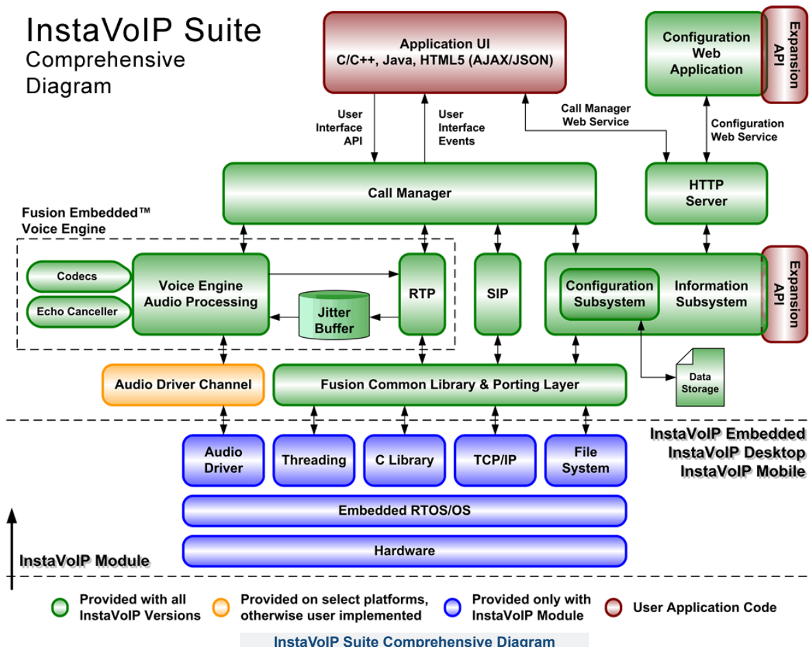
InstaVoIP Suite Comprehensive Diagram
